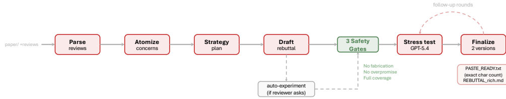
Figure 12: Workflow 4: Rebuttal. Seven phases from parsing reviews through stress-testing, with three safety gates.
